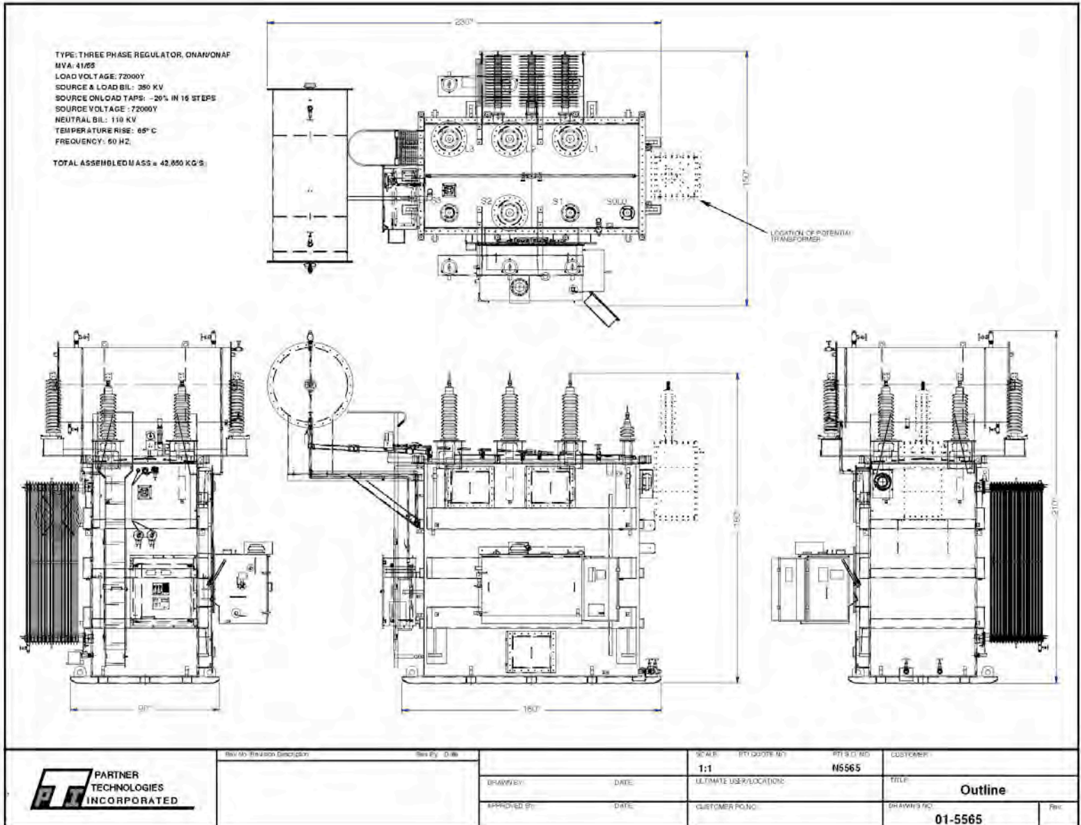
Typical Outline Drawing of a Three Phase 41/55 MVA 72kv Voltage Regulator
